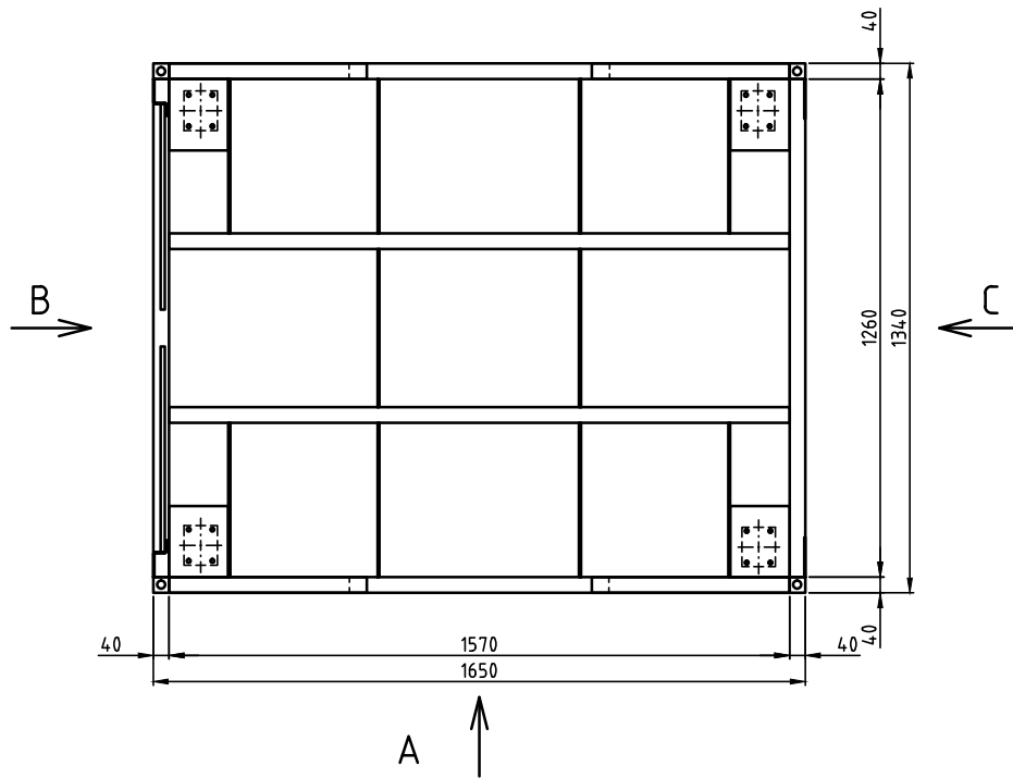
GROUND PLAN
