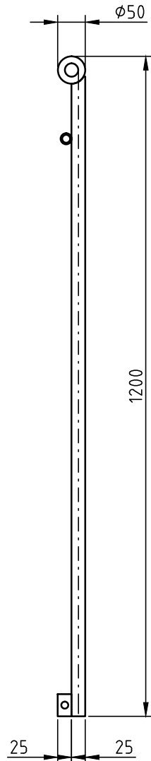
SIDE VIEW
